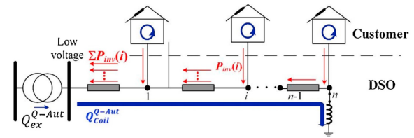
FIGURE 5. Active and reactive power flow in a low-voltage feeder with PV penetration that injects with \cos(\varphi) = 1 , the L(U) control strategy is employed, and Q-autarky is applied.
