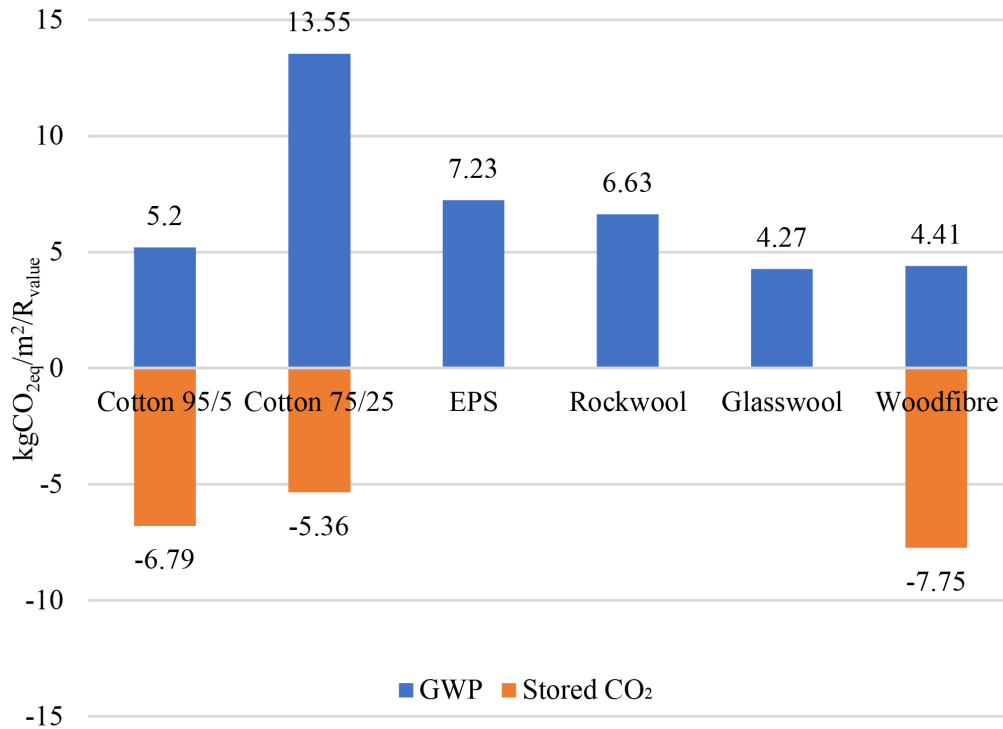
FIGURE 5. Carbon footprint (GWP) and CO 2 stored in 1 m 2 of textile and conventional insulation materials with a R T = 2.2 m 2 K/W.
