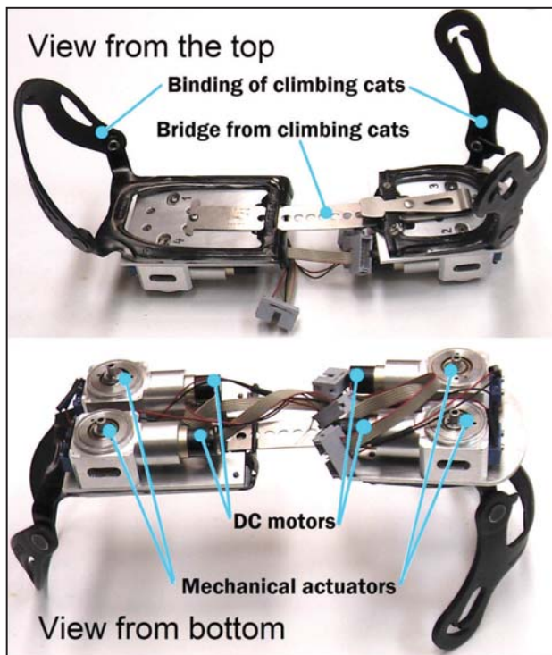
Fig. 1: Mechatronic rehabilitation shoes TUKE version [1].
