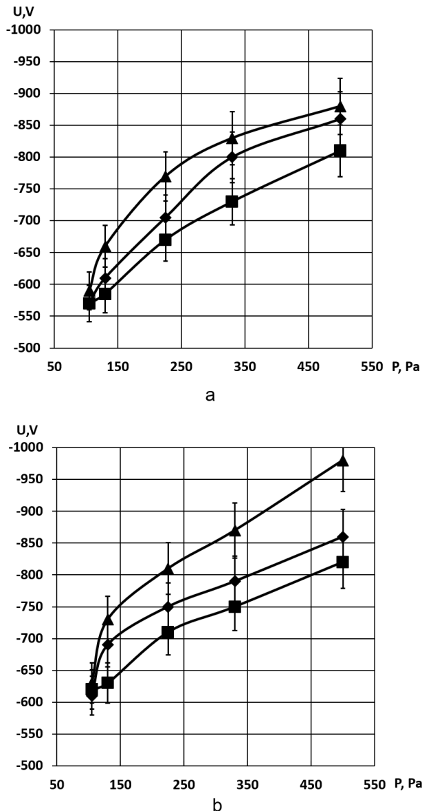
Figure 3. Values of excitation voltage of the discharge with hollow cathode effect in N_2 when the gas was fed past the discharge system (a), through the discharge system (b):
