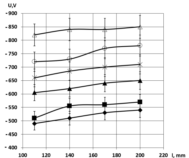
Figure 4. Values of excitation voltage of the discharge with hollow cathode effect when the distance between the cathode and the counter-electrode changes at different pressures:
