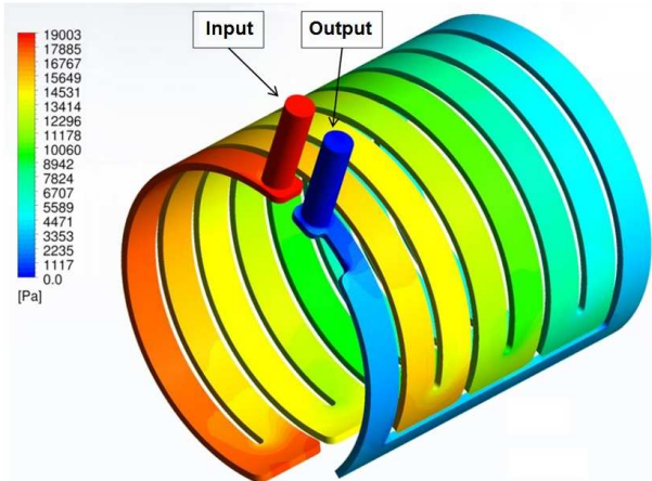
Fig. 15. Pressure field of the water inside water channel.
