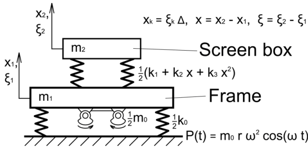
Fig. 2. Principal schema of the vibrating machine
