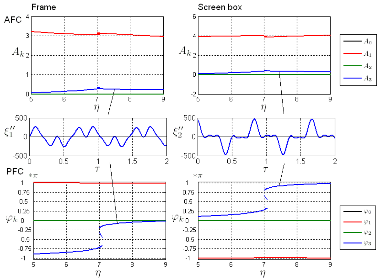
Fig. 5. Superharmonic resonance 3:1, k_{13} / k_{11} = 1
