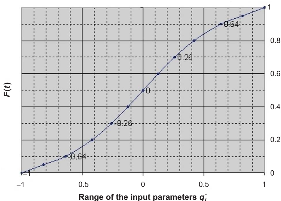
Fig. 2: Dividing the distribution function into intervals
