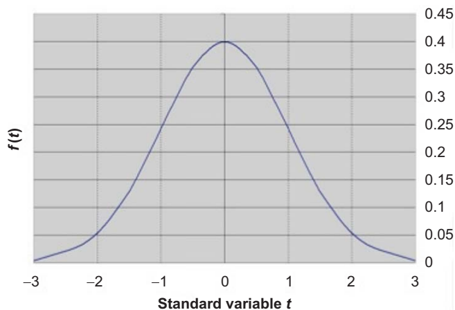
Fig. 1: Probability density function – Gaussian distribution
