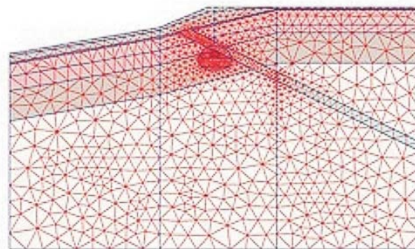
Fig. 4: Geometry of generated mesh in WTT km 5.160
