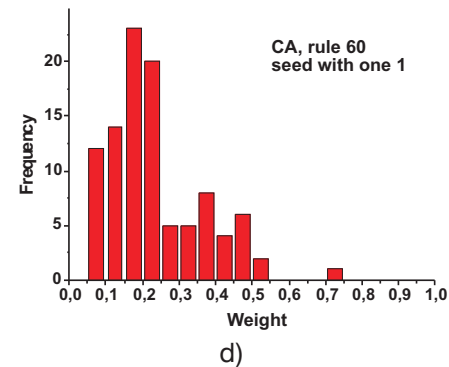
Fig. 10: a) distribution of weights for different PRPGs – LFSR with a balanced random seed, b) distribution of weights for different PRPGs – LFSR with an unbalanced random seed, c) distribution of weights for different PRPGs – CA with a balanced random seed, d) distribution of weights for different PRPGs – CA with an unbalanced random seed
