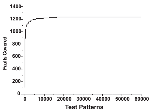
Fig. 6: Fault coverage curve
