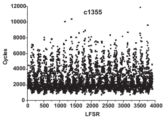
Fig. 5: Influence of the LFSR
