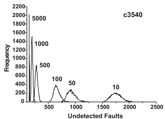
Fig. 7: Pseudo-random fault coverage
