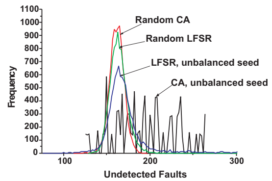
Fig. 9: Fault coverage of a “specially” seeded CA and LFSR
