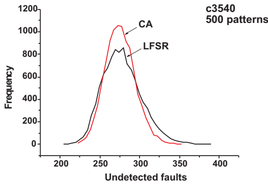
Fig. 8: Comparison of the fault coverage obtained by LFSR and CA
