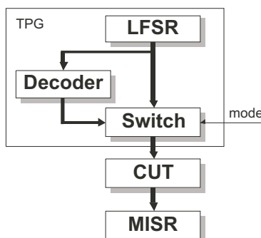
Fig. 11: Mixed-mode BIST structure
