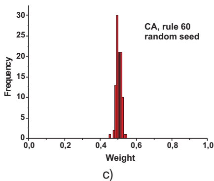
Fig. 10: a) distribution of weights for different PRPGs – LFSR with a balanced random seed, b) distribution of weights for different PRPGs – LFSR with an unbalanced random seed, c) distribution of weights for different PRPGs – CA with a balanced random seed, d) distribution of weights for different PRPGs – CA with an unbalanced random seed
