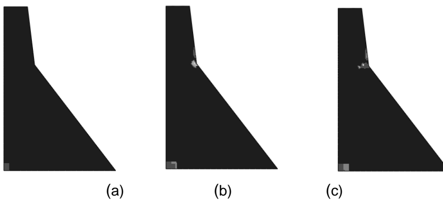
Fig. 2 - Failure modes of the Koyna dam
