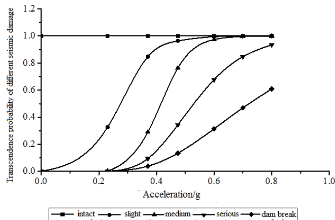
Fig. 7 - Seismic vulnerability curves of the Koyrna dam considering strain rate
