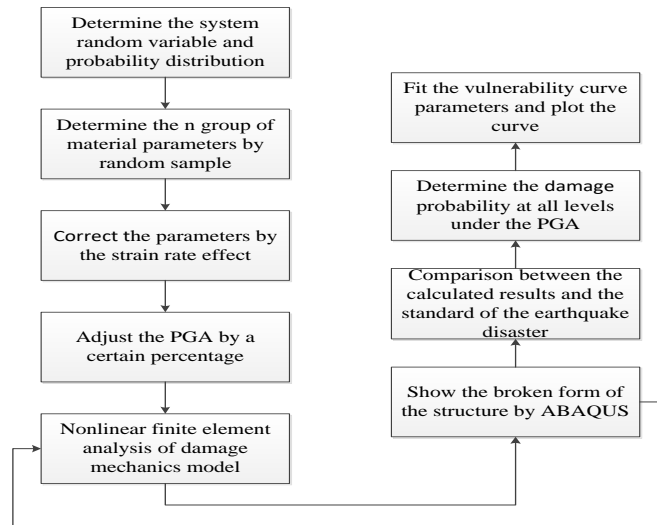
Fig. 5 - Procedure of seismic vulnerability analysis
