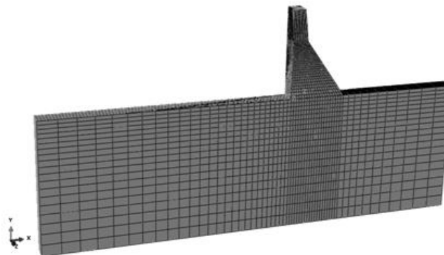
Fig. 1 - Model of Koyna dam
