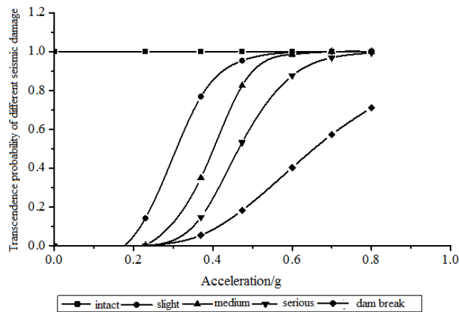
Fig. 6 - Seismic vulnerability curves of the Koyrna dam without considering strain rate
