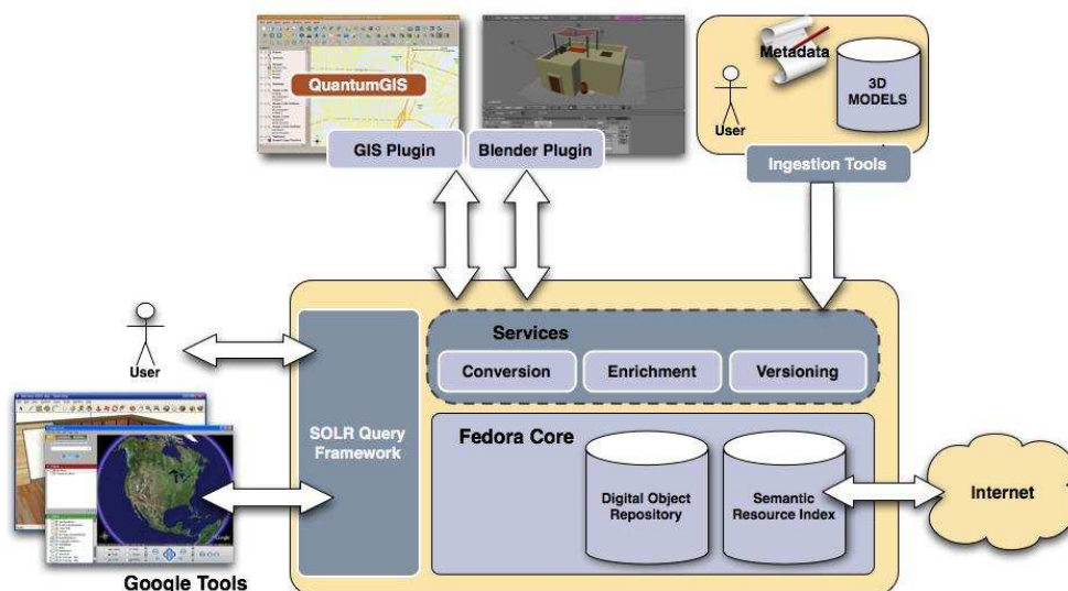
Figure 1: The structure of our 3D digital repository
